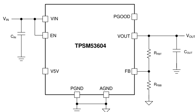
Simplified Schematic
