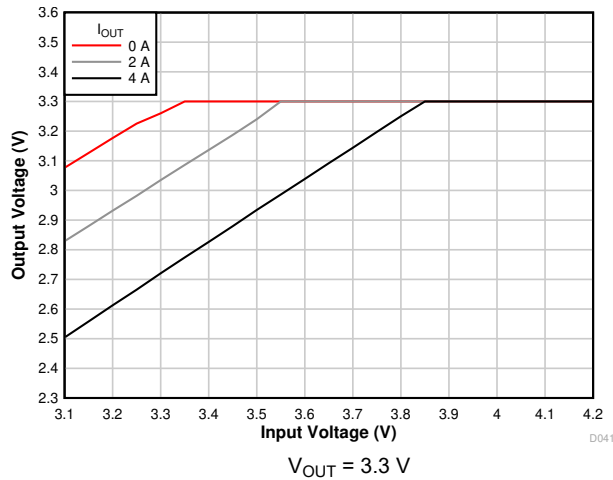
Figure 7-7. Voltage Dropout
