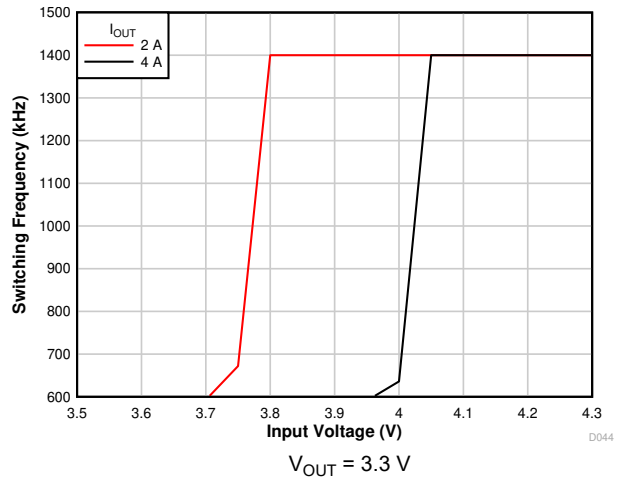
Figure 7-8. Frequency Foldback
