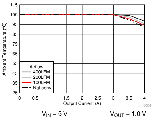
Figure 6-5. Safe Operating Area
