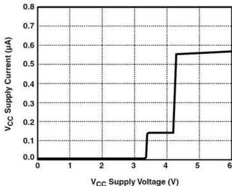
Figure 1. Supply Current vs. Voltage ( V_{AUX} = 3.3\text{ V} )
