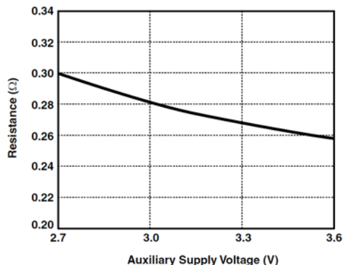
Figure 2. Switch Resistance vs. Supply Voltage
