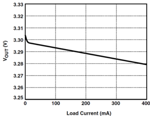
Figure 5. Load Regulation
