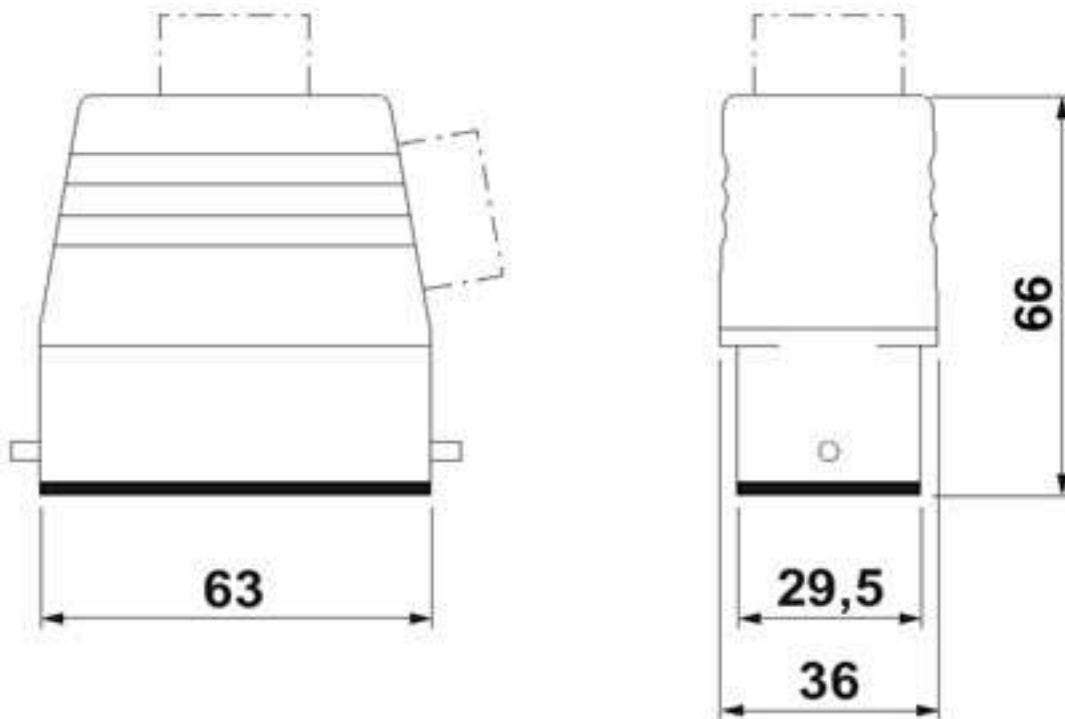
Dimensioned drawing
