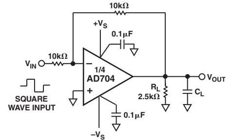
TPC 21a. Unity Gain Inverter Connection
