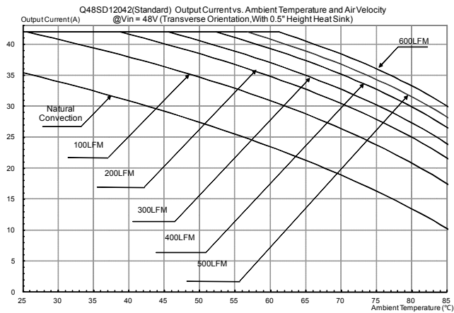
Figure 27: Output current vs. ambient temperature and air velocity @Vin=48V(Transverse Orientation, airflow from Vin+ to Vin-,with 0.5" height heat sink)
