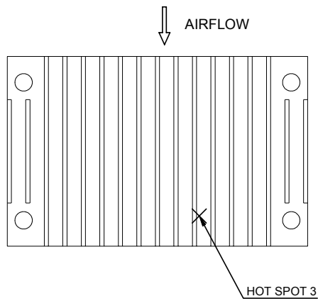
Figure 26: * Hot spot 3 temperature measured point
