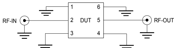
Fig 1. Block diagram of Test Circuit used for characterization, Test board TB-QAT-4C+ Conditions: Attenuation, VSWR: Pin=0 dBm
