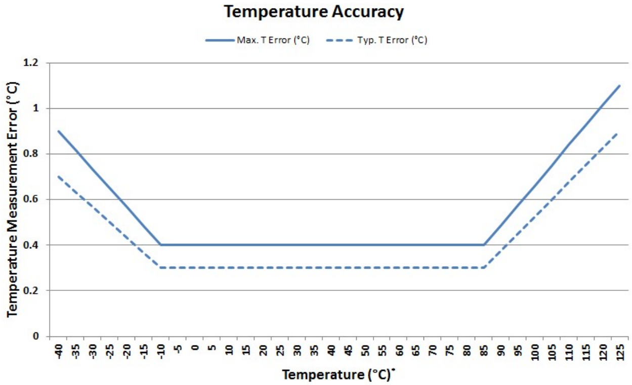
Figure 3. Temperature Accuracy*
