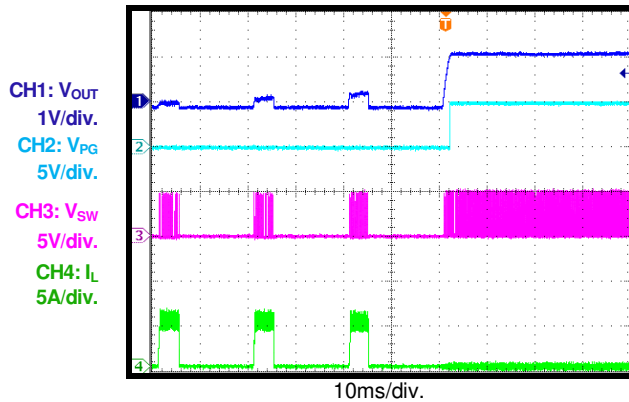
Short-Circuit Recovery PWM
