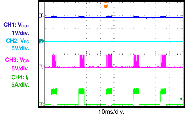
Short-Circuit Entry PFM
