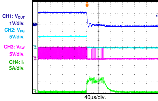
Short-Circuit Entry PWM
