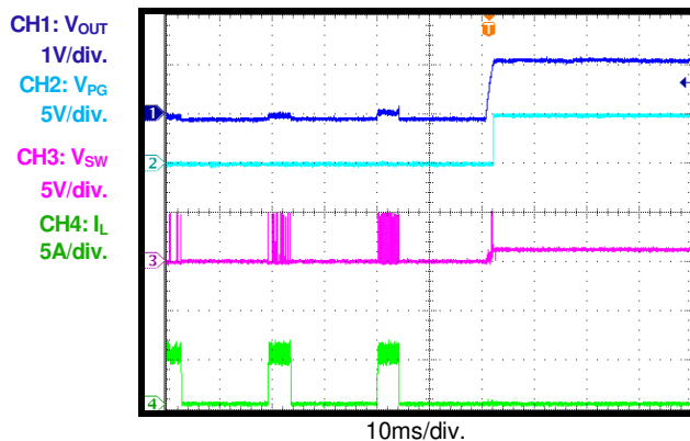
Short-Circuit Recovery PFM
