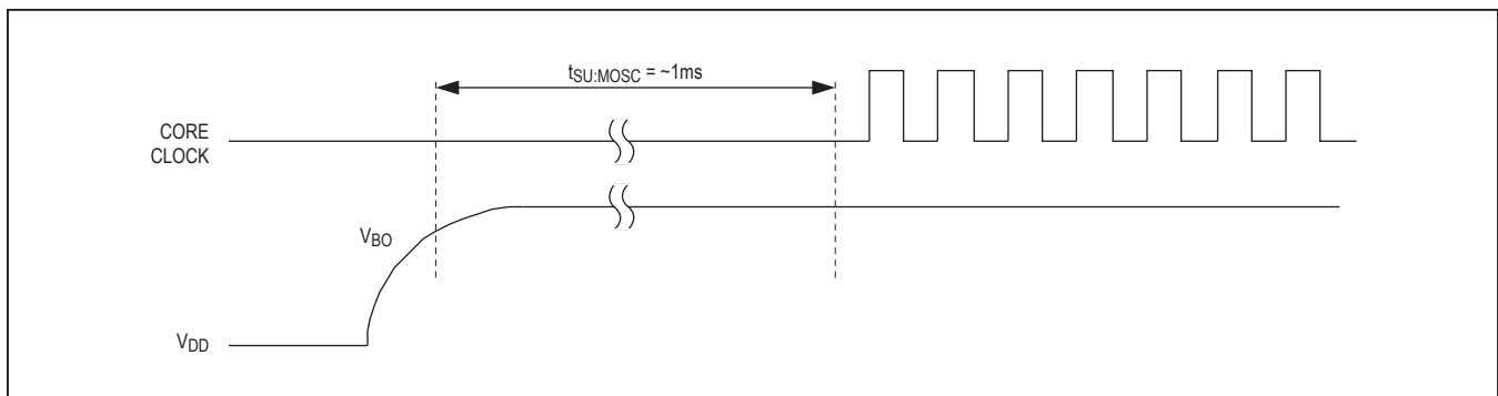
Figure 8. System Timing
