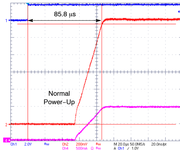
Figure 26. Normal Power Up, V_{OUT} = 1.225\text{ V}
