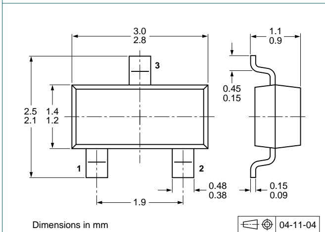
Fig 14. Package outline PDTC143ZT (SOT23)
