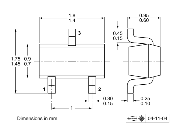
Fig 12. Package outline PDTC143ZE (SOT416/SC-75)
