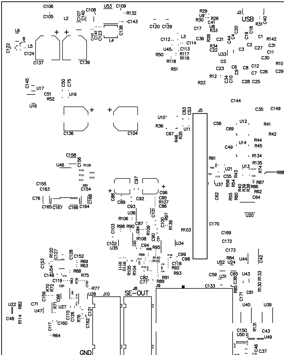
Figure 29. PPC3-EVM-MB Bottom Silk Screen
