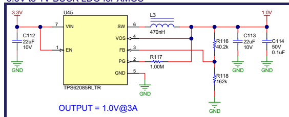
3.3V to 1V BUCK LDO for XMOS
