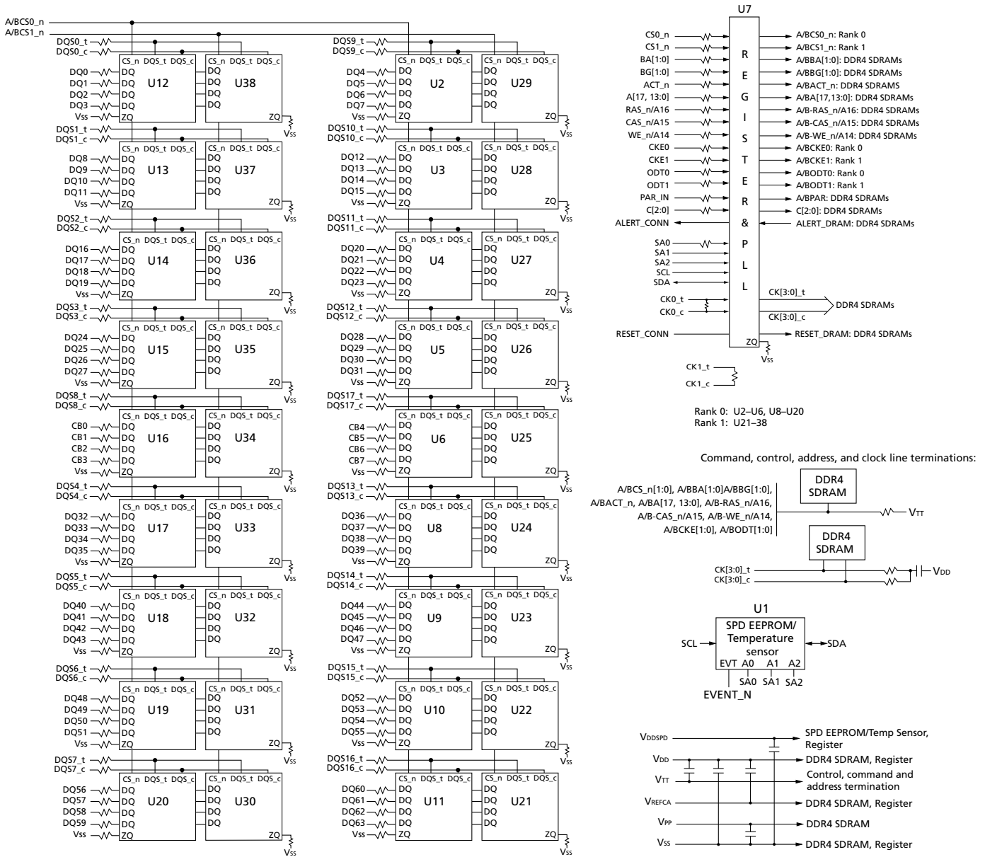
Figure 4: Functional Block Diagram, R/C-B2 (PCB 1971)
