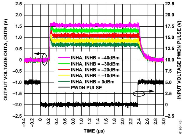
Figure 48. Output Response Using Power-Down Mode for Various RF Input Levels, Carrier Frequency = 900 MHz, CLPA = 0.1 μF
