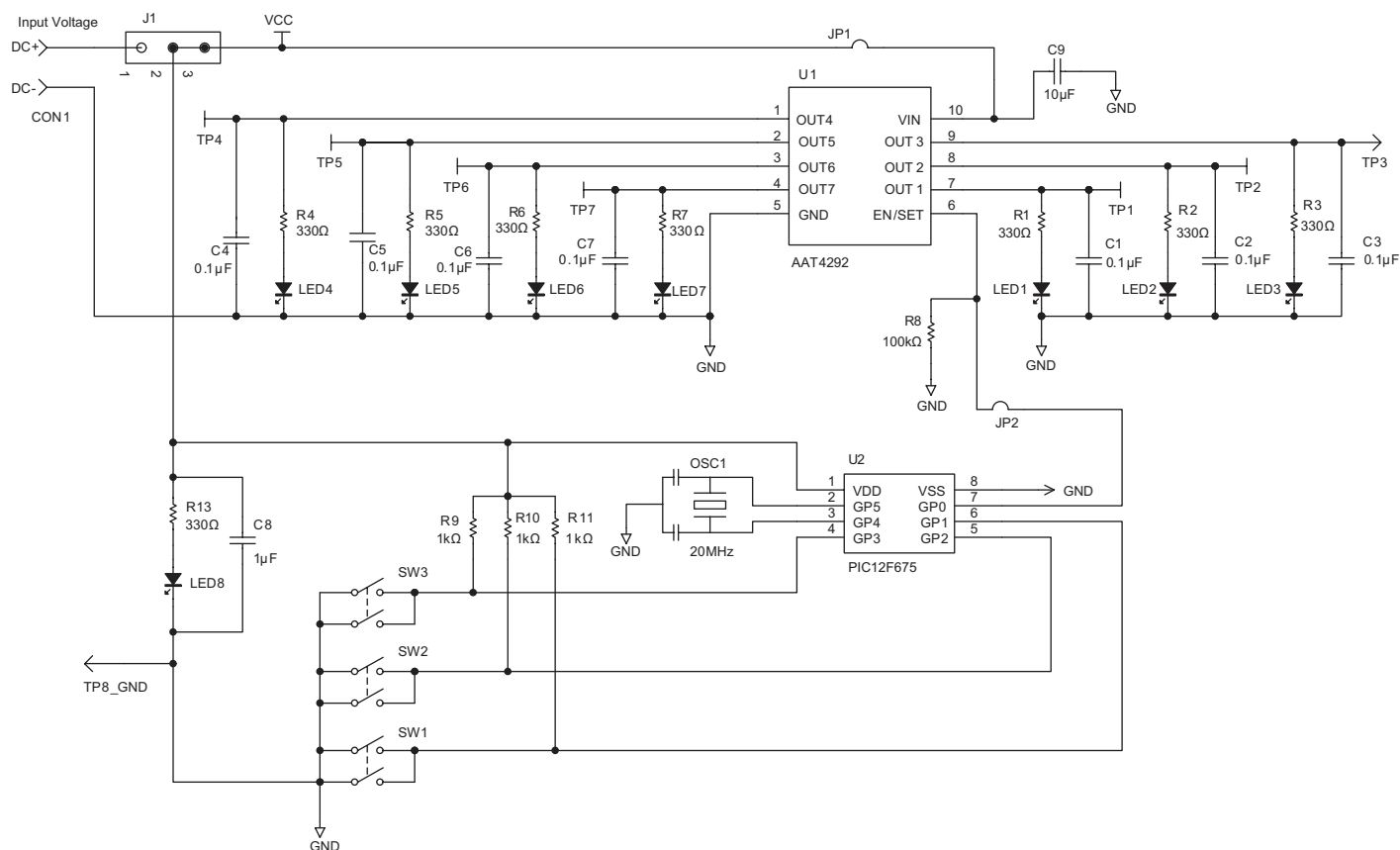
Evaluation Board Schematic
