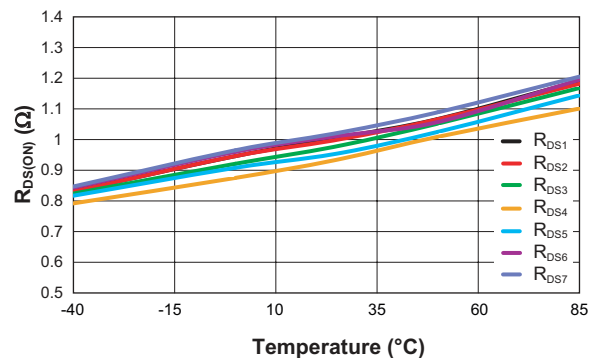
R_{DS(ON)} vs. Temperature ( V_{IN} = 5.0V ; I_{OUT1-7} = 10mA )
