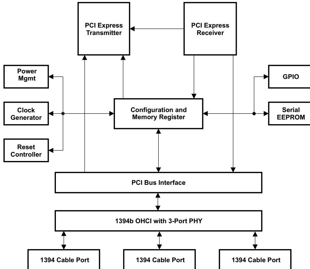
Figure 3-1. XIO2213A Block Diagram
