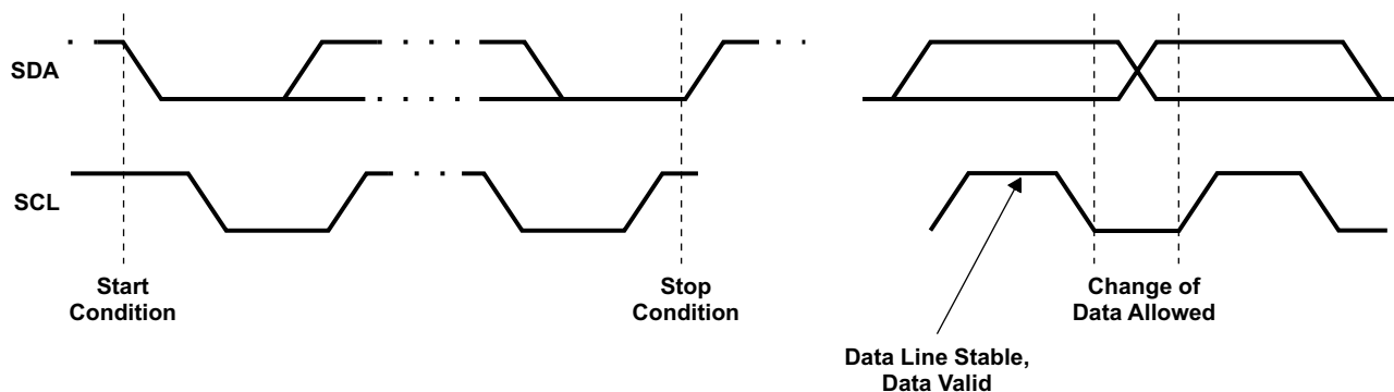
Figure 3-7. Serial-Bus Start/Stop Conditions and Bit Transfers
