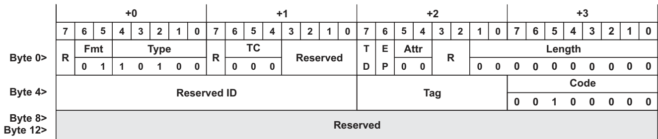
Figure 3-4. PCI Express ASSERT_INTA Message
