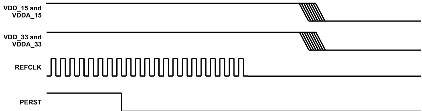
Figure 3-3. Power-Down Sequence
