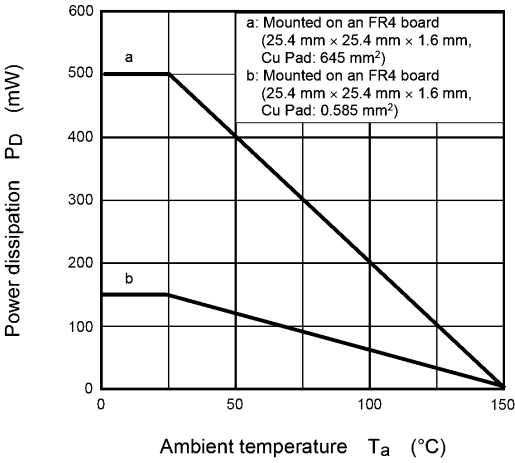
Fig. 8.14 P_D - T_a
