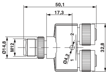
Dimensioned drawing
