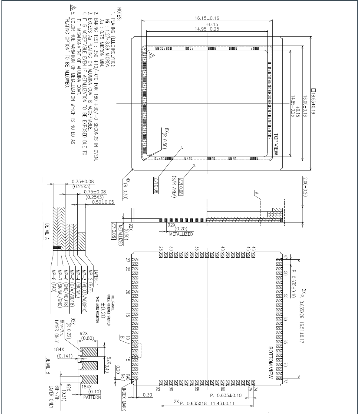
Figure 102: LCC Package Drawing
