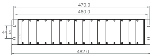
Panel View
