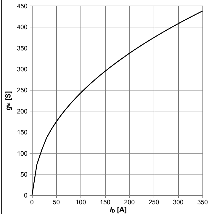
Diagram 8: Typ. transconductance
