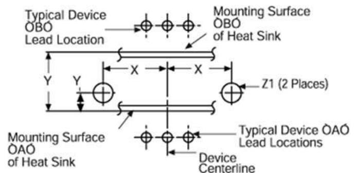
Mounting Details:
