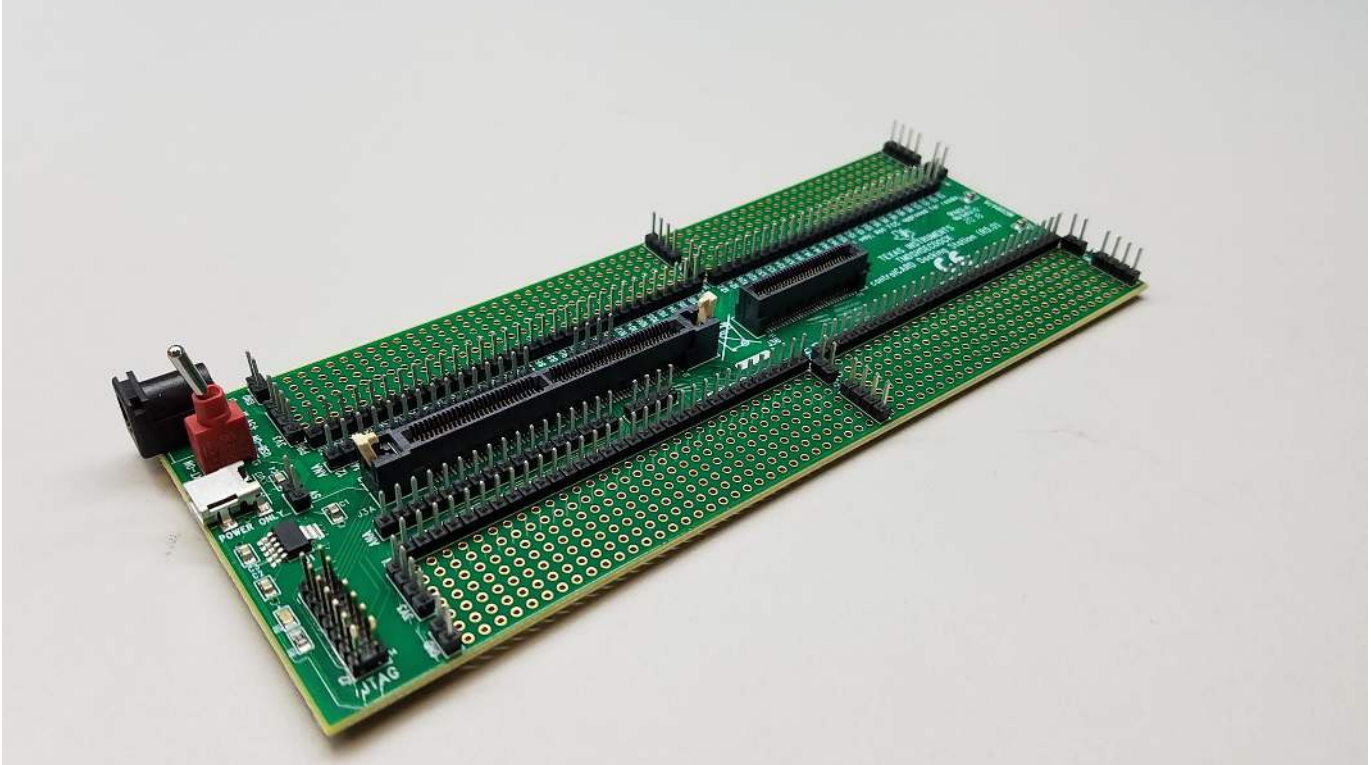
Figure 1-1. 180-Pin controlCARD Docking Station (Revision 5.0 shown)
