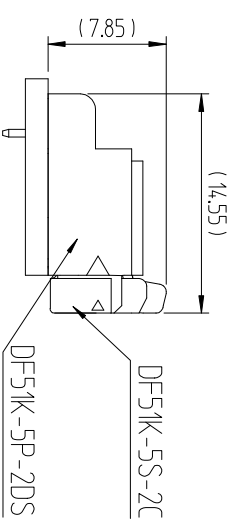
ENGAGEMENT FIGURE (2:1)
