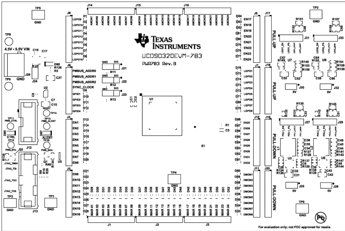
Figure 11. Top Overlay
