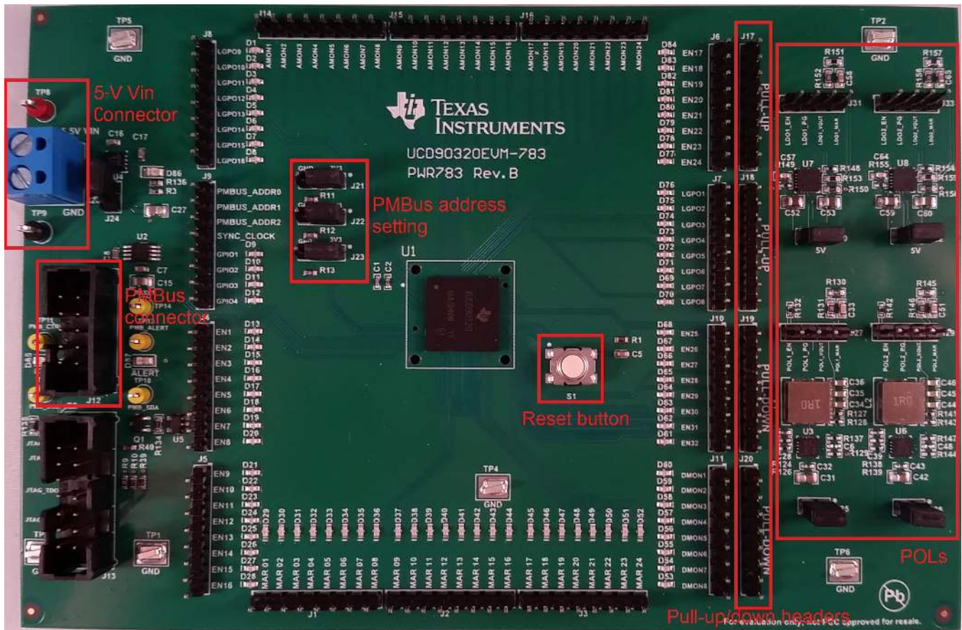
Figure 1. UCD90320EVM-783
