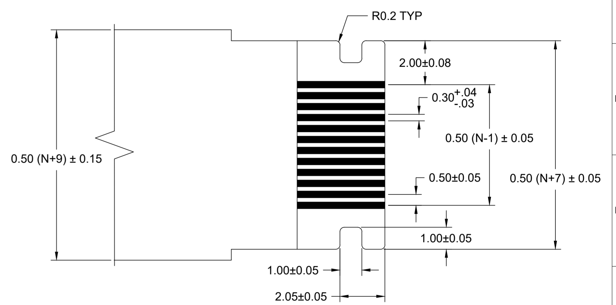
END-TAIL DIMENSIONS SCALE 10:1
