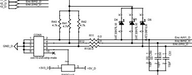
Figure 5. Driver board schematics - sensing and status
