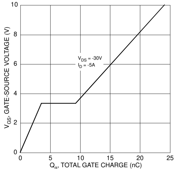
Figure 12 Gate-Charge Characteristics
