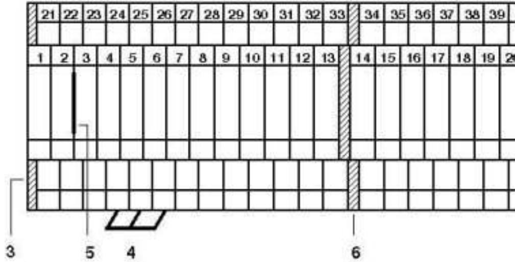
Circuit diagram
