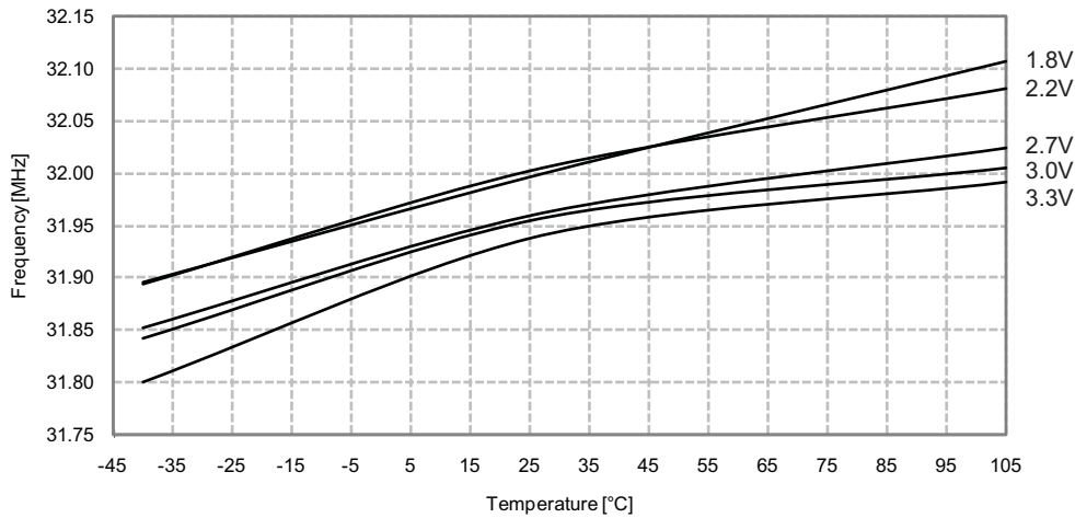
Figure 36-60. 32MHz Internal Oscillator Frequency vs. Temperature DFLL enabled, from the 32.768kHz internal oscillator
