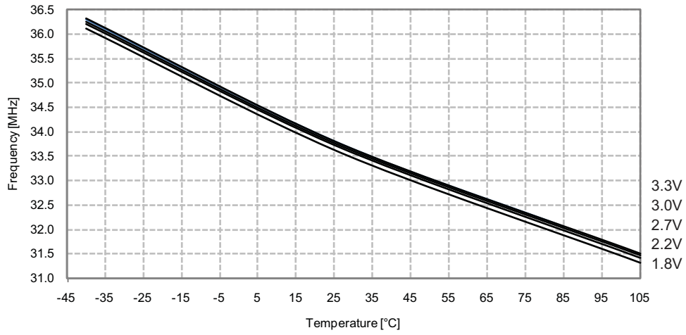
Figure 36-59. 32MHz Internal Oscillator Frequency vs. Temperature DFLL disabled
