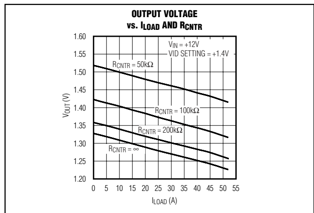
Figure 5. Output Voltage vs. I LOAD and RCNTR
