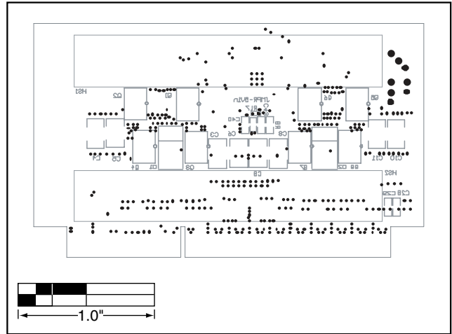
Figure 24. MAX5037 EV Kit Component Placement Guide—Solder Side
