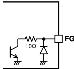
5) Speed pulse signal output terminal
