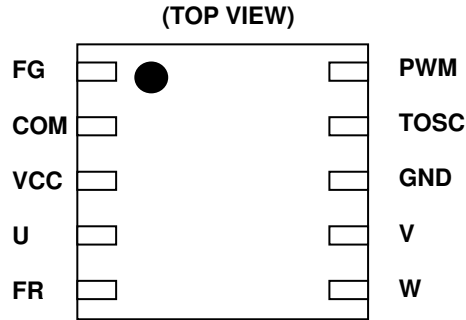
Figure 1. Pin Configuration
