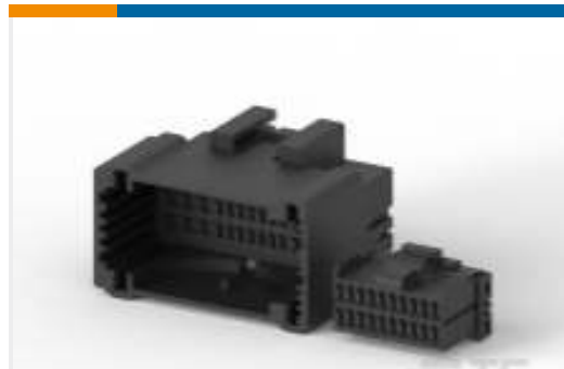
TE Part #936092-1 MULTILOCK, CONNECTOR HOUSING
