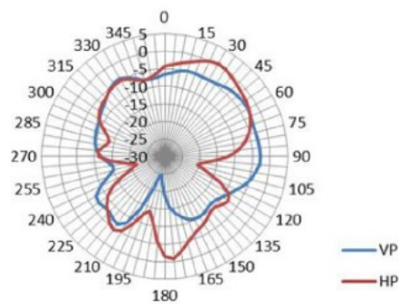
H Plane
