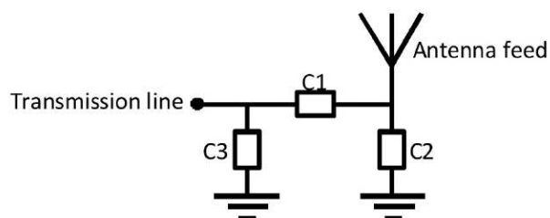
Matching circuit
