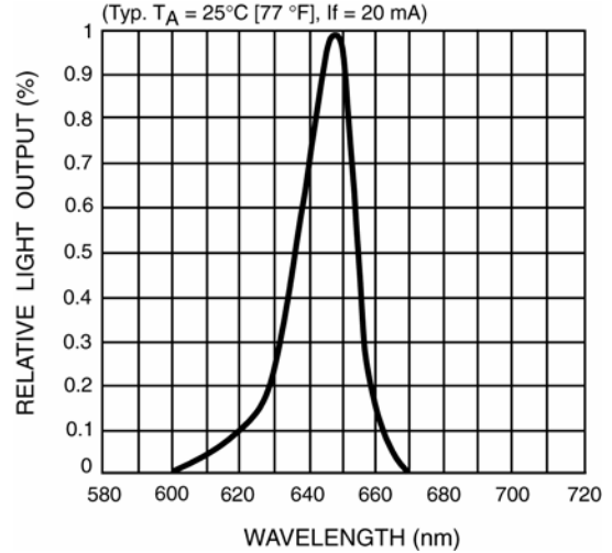
FIGURE 2. TYPICAL EMISSION SPECTRUM
