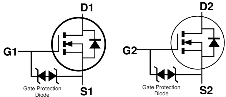
Internal Schematic
