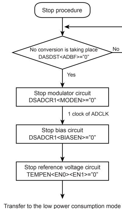
Figure 14-3 Stop procedure
