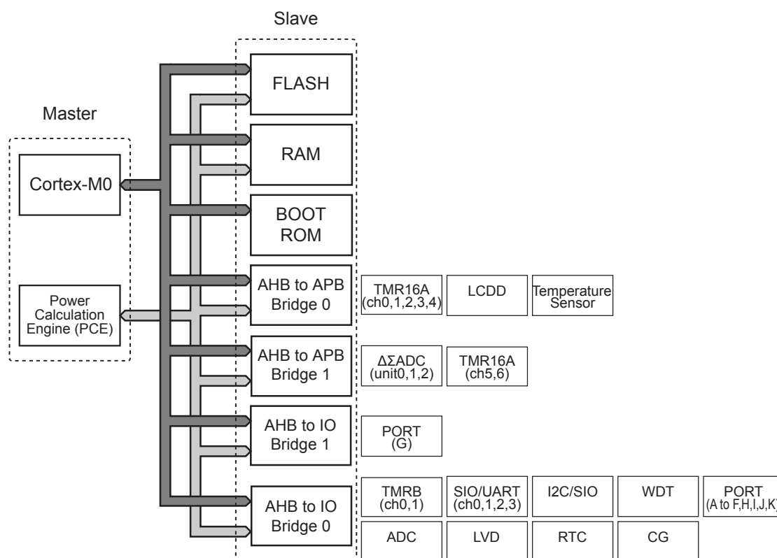
Figure 4-2 Bus structure
