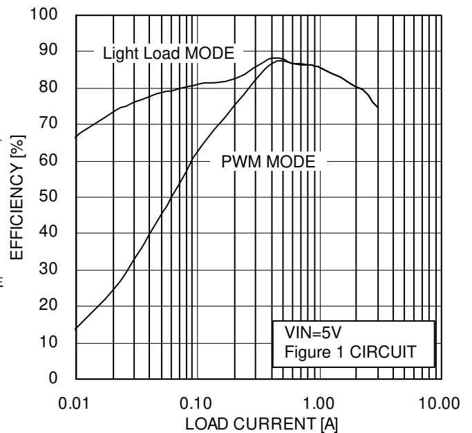
Figure 2. Efficiency (BD90525EFJ-C)
