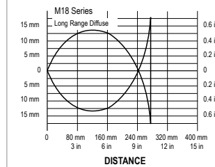
Beam Pattern
