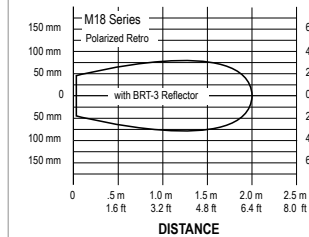
Beam Pattern
