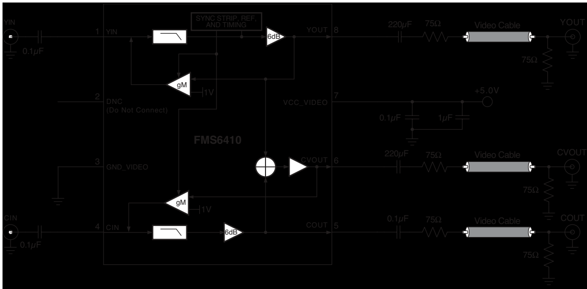
Figure 1. Typical Configuration
