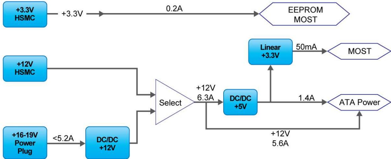
Figure 4-11 Power Tree
