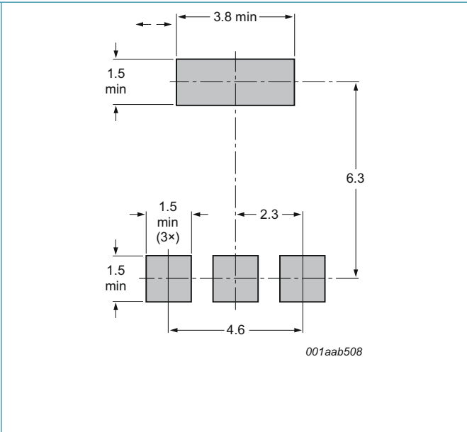
Fig. 8. Minimum footprint SOT223
