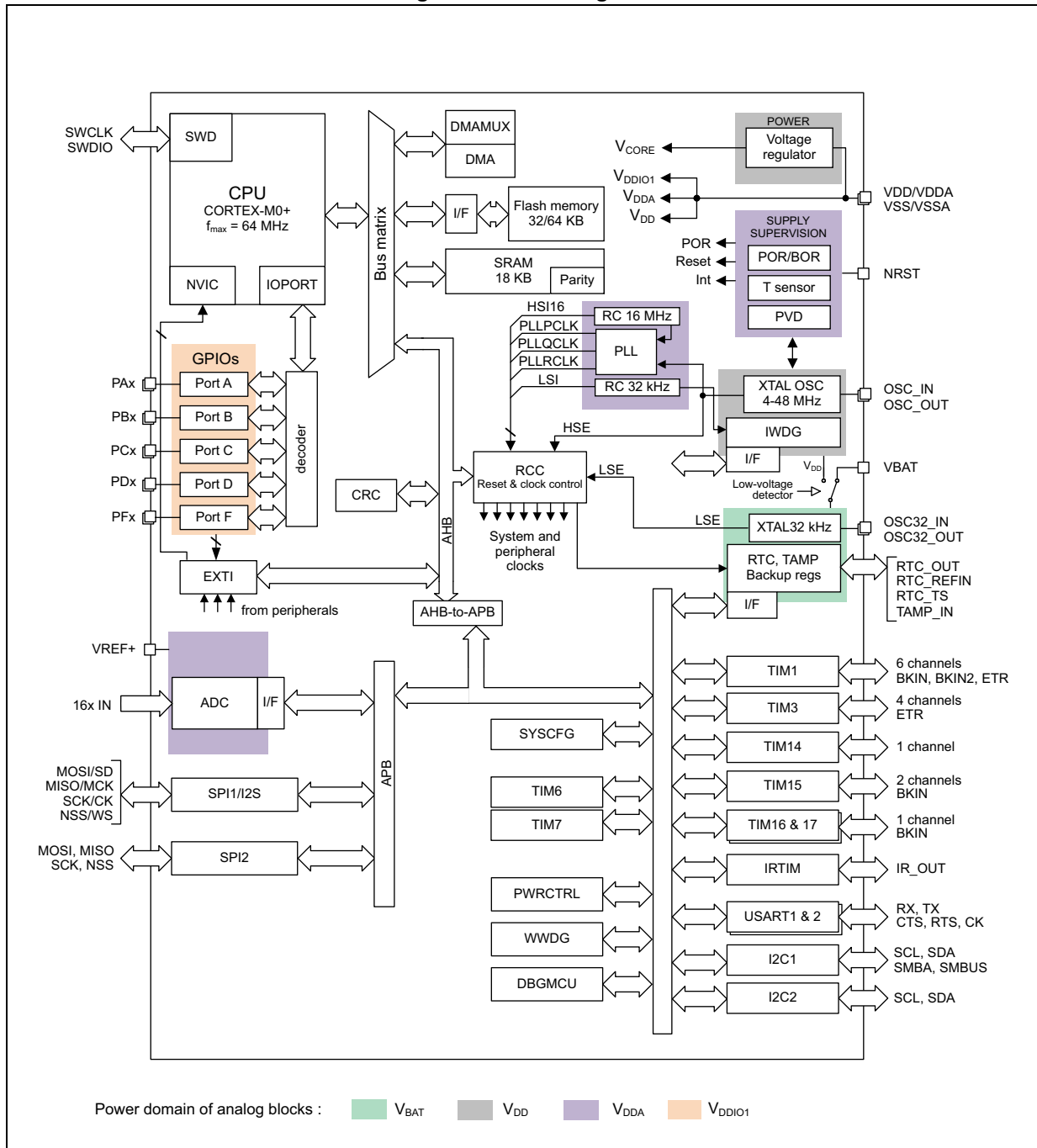
Figure 1. Block diagram
