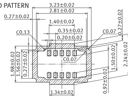
SOLDER RESIST
