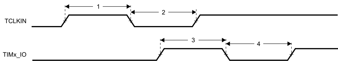
Figure 8-97. Timer Timing
