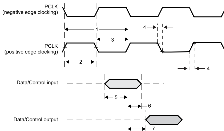
Figure 8-47. ISSCAM Timings
