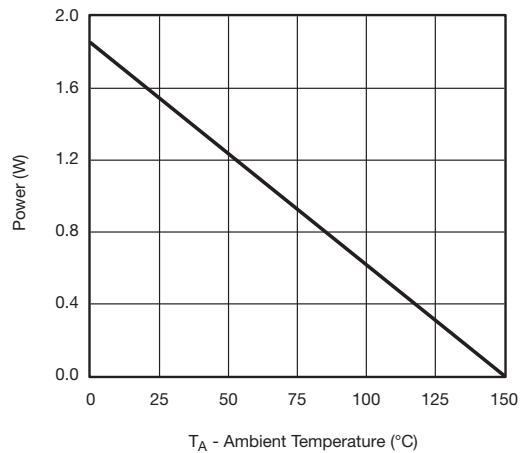
T A - Ambient Temperature (°C) Power, Junction-to-Ambient
