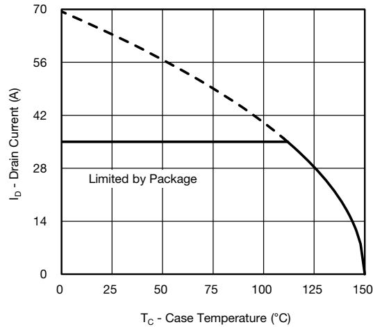
T C - Case Temperature (°C) Current Derating a
