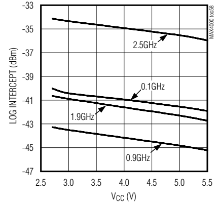
MAX4002 LOG INTERCEPT vs. V_{CC} (UCSP)
