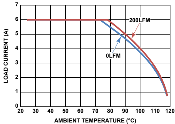
FIGURE 29. DERATING CURVES AT V_{IN} = 3.3V , V_{OUT} = 1V
