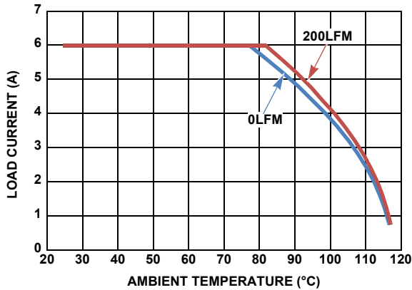
FIGURE 27. DERATING CURVES AT V_{IN} = 5V , V_{OUT} = 1V
