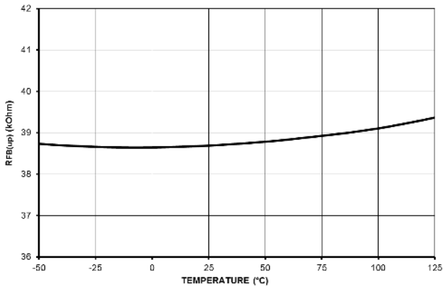
Figure 15. FB Pin Internal Pull-up Resistor R_{FB(up)}
