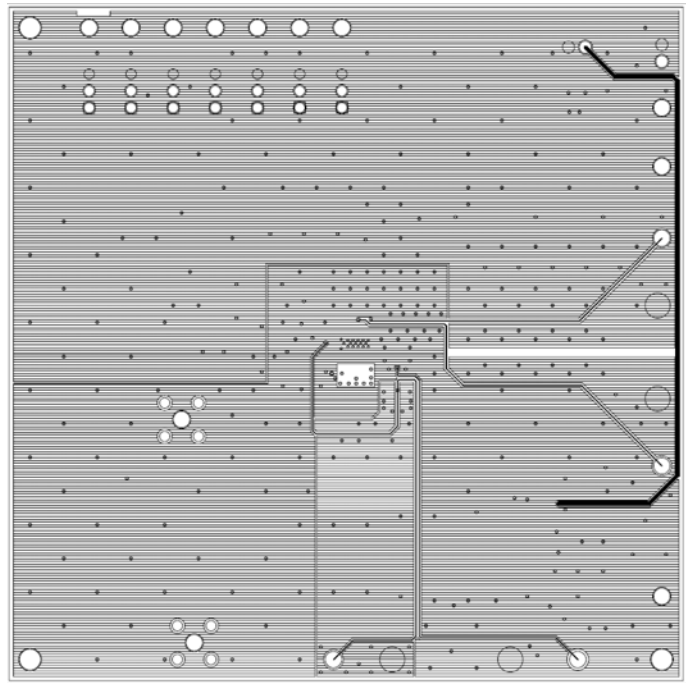
FIGURE 6. INTERNAL LAYER 2
