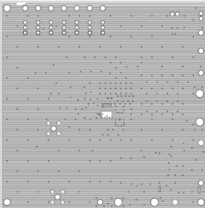
FIGURE 5. INTERNAL LAYER 1
